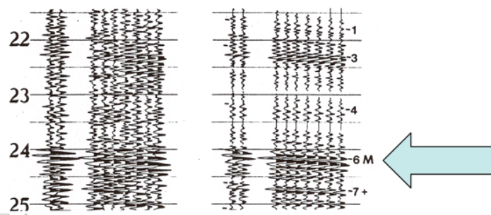
Wide-angle reflections generated by a quarry blast in the central Appalachians, recorded with a short-aperture array (blast duration: ~0.25 seconds; center distance: ~124 km). Before (left) and after (right) coherency filtering. Event "M" (center-offset travel time: ~24 s), interpreted as a reflection from the uppermost mantle, migrates to a depth of ~54 km beneath the Conestoga Valley of southeastern Pennsylvania (Hawman & Phinney, 1992b).
